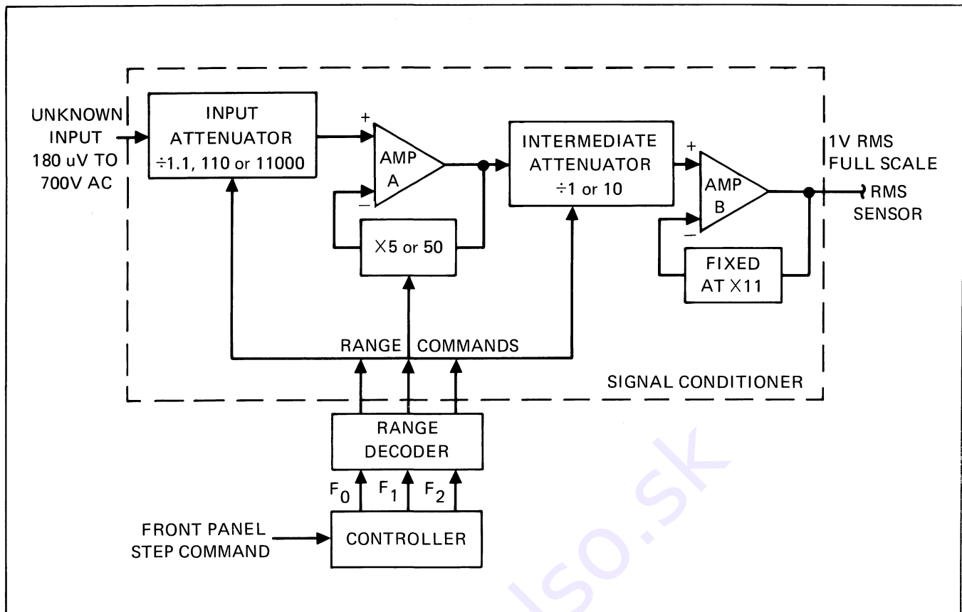
Figure 3-3. Signal Conditioner
