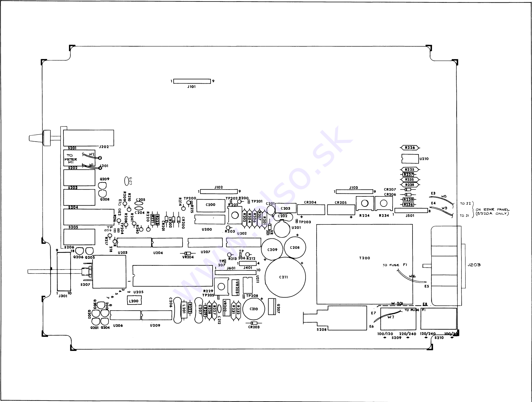
Figure 5-2. A1 8920A Main PCB Assembly (cont)
